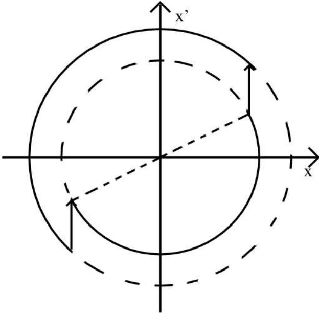
Figure 2: Beam-beam compensation concept. The nonlinear beam-beam kick experienced in the collision with an oncoming proton beam is exactly compensated after a betatron phase advance of 180 degrees by colliding with an electron beam of equal density distribution.
