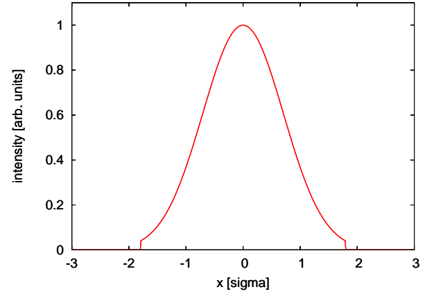
Figure 4: Transverse profile of the Gaussian electron lens beam with its sharp edge at the cathode radius. For better visibility, a cathode radius of 1.8\sigma is shown here.
