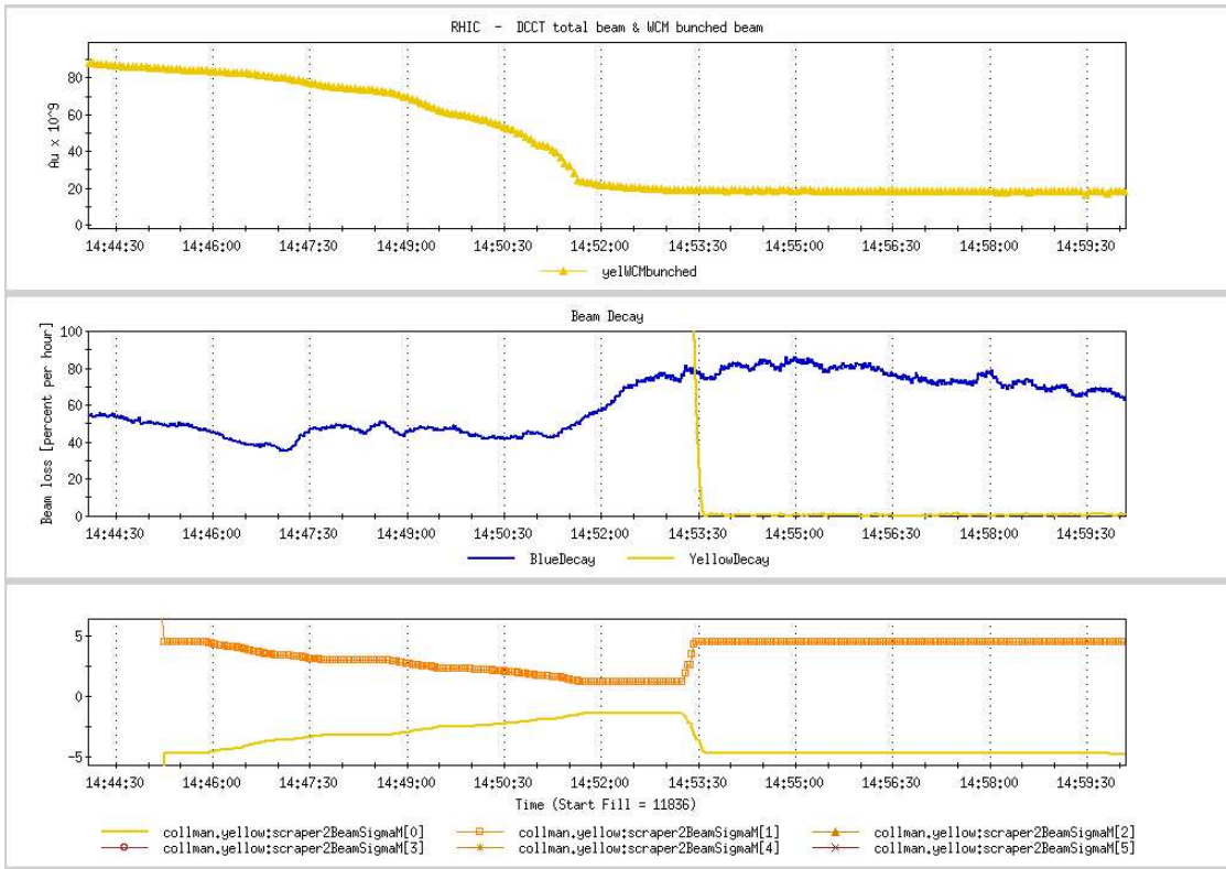
Figure 5: Yellow beam intensity, Blue hourly beam decay, and Yellow collimator position vs. time during aggressive scraping of the Yellow beam.
