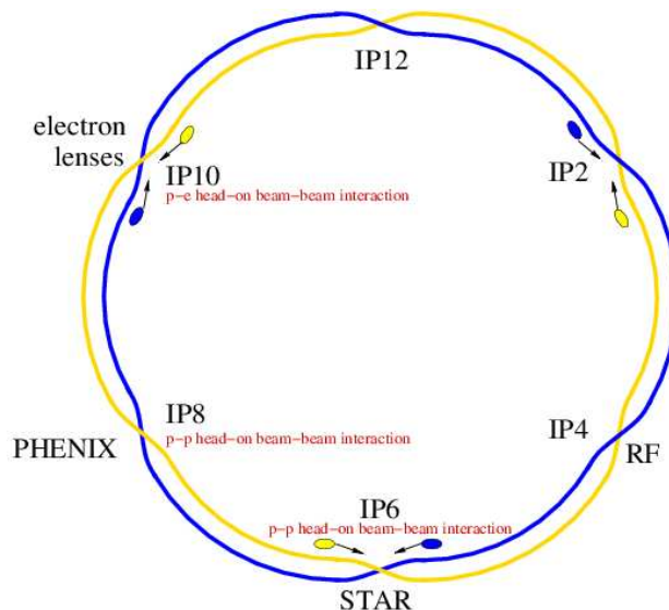
Figure 1: Schematic view of RHIC. Beams collide in IPs 6 and 8. IP 10 will be equipped with an electron lens for head-on beam-beam compensation.
