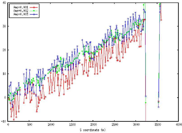
Figure 3: Measured accumulated phase shift \Delta Q(s) = \Delta\psi(s)/(2\pi) around the ring, vs. longitudinal position s .
